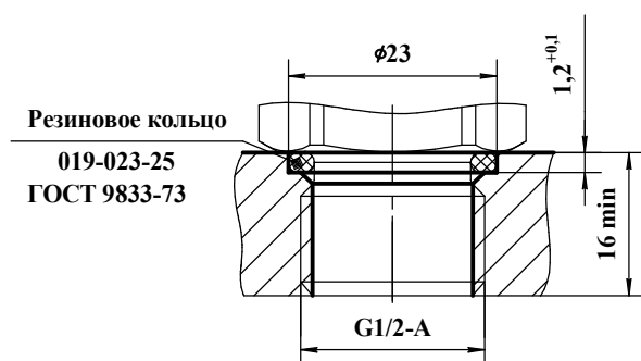
PTM-M-1(2)-MO-G-1(1,6...6)-...-G1
