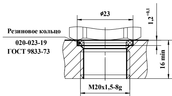
PTM-M-1(2)-MO-G-1(1,6...6)-...-M1
